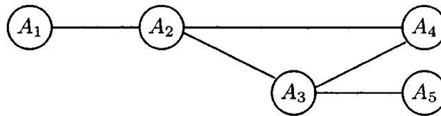
Figure 1. A constraint graph.
