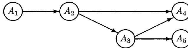
Figure 2. A directed constraint graph.
